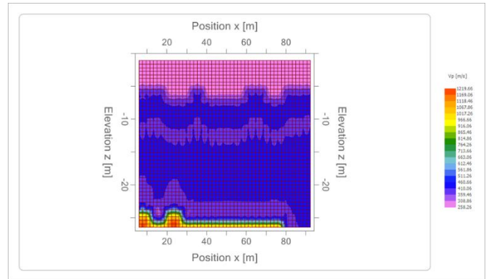
Figure 16: Velocity Map of the Subsurface in Okorikperhe
