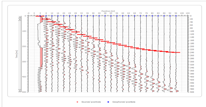
Figure 18: 2 nd Shot at Arrival in Okukuoko
