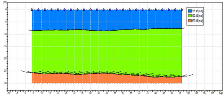
Figure 23: Morphology of the Subsurface Refractors in Okukuoko
