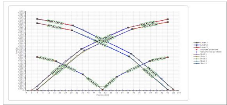
Figure 22: Travel Time Curve in Okukuoko
