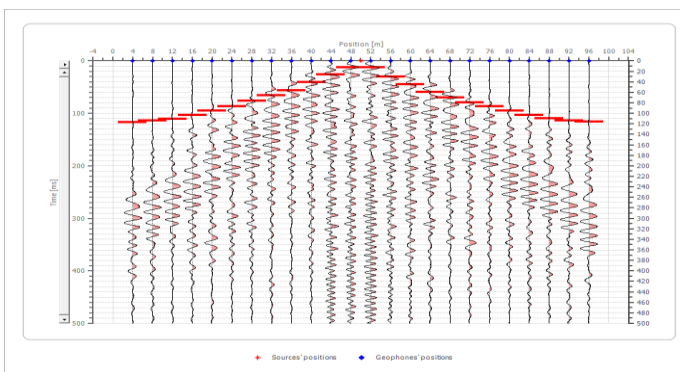
Figure 19: 3 rd Shot at Arrival in Okukuoko
