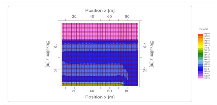
Figure 24: Velocity Map of the Subsurface in Okukuoko
