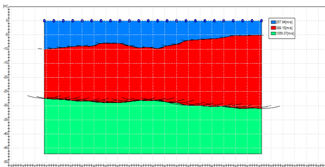
Figure 7: Morphology of the Subsurface Refractors in FUPRE-campus
