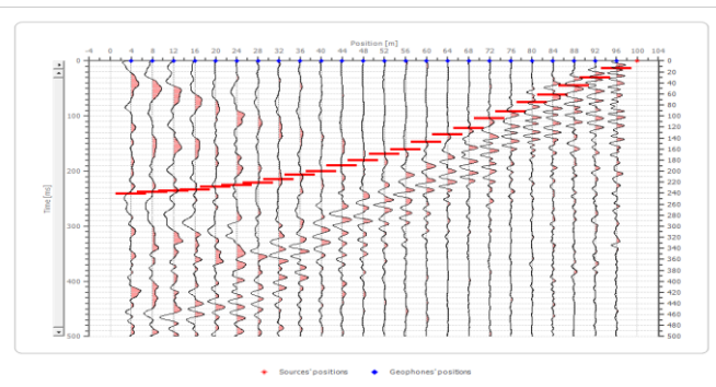
Figure 13: 5 th Shot at Arrival in Okorikperhe
