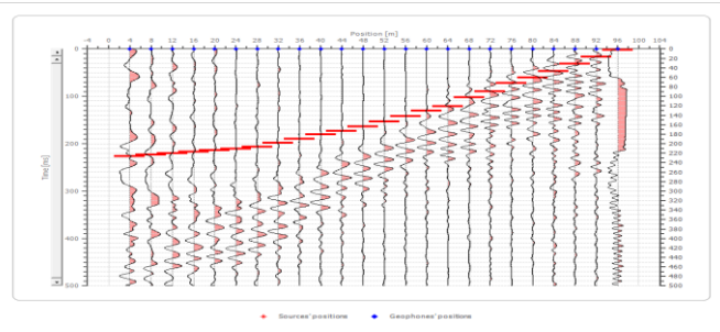
Figure 12: 4 th Shot at Arrival in Okorikperhe
