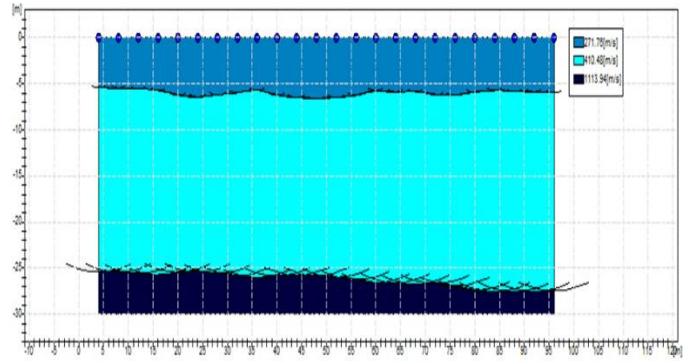
Figure 15: Morphology of the Subsurface Refractors in Okorikperhe
