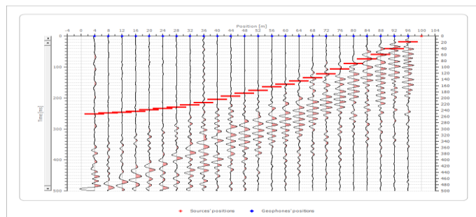
Figure 21: 5 th Shot at Arrival in Okukuoko
