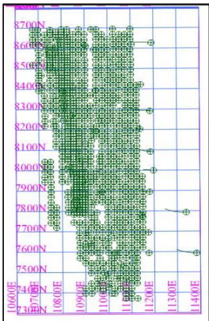
Figure 3: Borehole location plan
