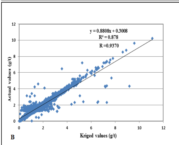
Figure 7: Scatter plot of actual on kriged values, (A) A reef, (B), CDE reef
