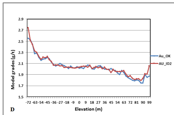
Figure 13: Comparison of estimated grades: (A) OK, ID, ID 2 , ID 3 , and ID 4 model for A reef, (B) OK, ID, ID 2 , ID 3 , and ID 4 model for CDE reef, (C) OK and ID 2 model for A reef, (D) OK, and ID 2 model for CDE reef.
