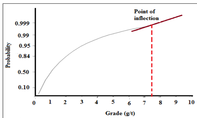
Figure 9: Example of probability plots, the case for A Reef
