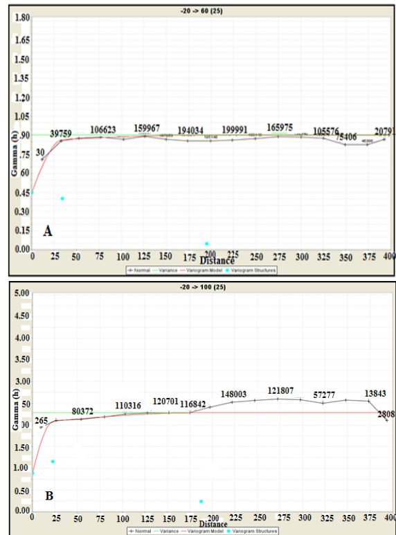
Figure 10: Examples of directional variograms: (A) A along 60°, (B) CDE along 100°
