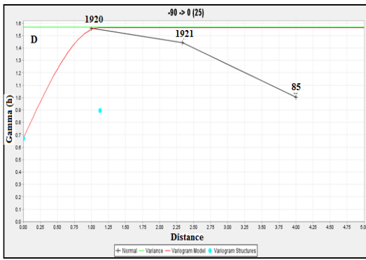
Figure 6: Fitted experimental downhole semi-variograms for the reefs: (A) A-Reef, (B) CDE-Reef, (C) F-24 Reef, and (D) G-Reef.
