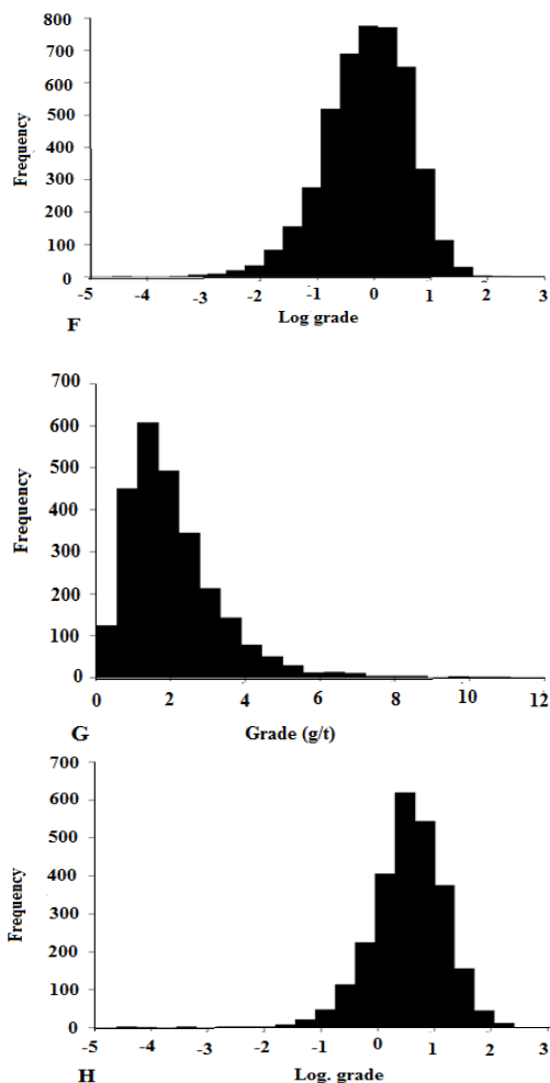
Figure 8: Plots of the histograms of the raw data and logarithms of grades for the separate reefs: (A) Frequency distributions of Au grades for A reef, (B) Logarithms of grade for A reef, (C) Frequency distributions of Au grades for CDE reef, (D) Logarithms of grade for CDE reef, (E) Frequency distributions of Au grades for F24 reef, (F) Logarithms of grade for CDE reef, (G) Frequency distributions of Au grades for G reef, (H) Logarithms of grade for G reef
