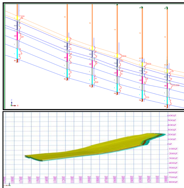
Figure 4: (a) Section 7625N of the Study Area and (b) 3D wireframe solids generated
