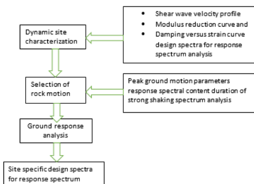
Figure 2: Site specific ground response analysis (Govindaraju L. et al. 2004)
